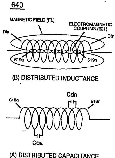
FIGURE 7-3: COIL INTERACTION
